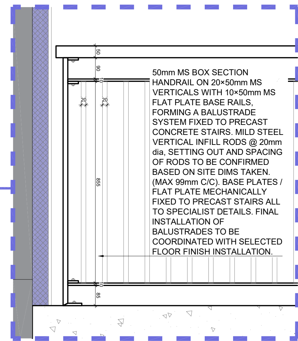
9 63.01 HANDRAIL / BALUSTRADE DETAIL SCALE: 1:10
